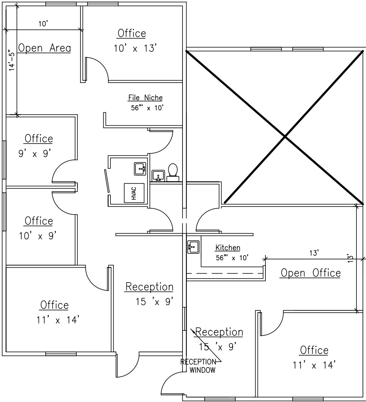
3960 A1 - 1,728 sf
